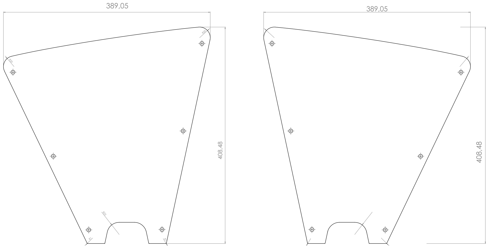
Side panel (2x)
