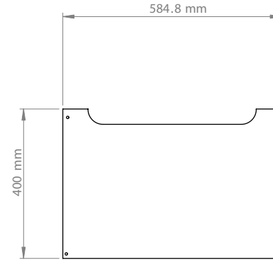
Front panel
